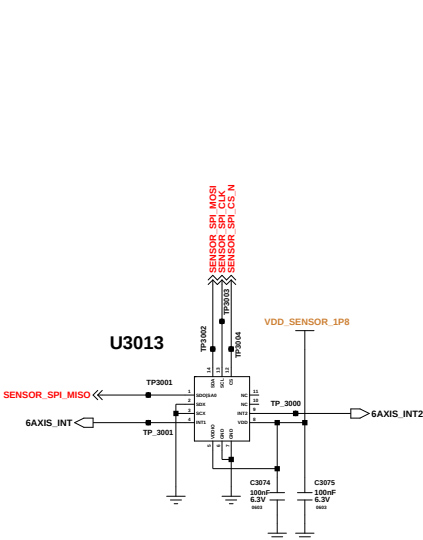
6 AXIS(ACC+GRYO) STM(3x2.5)
