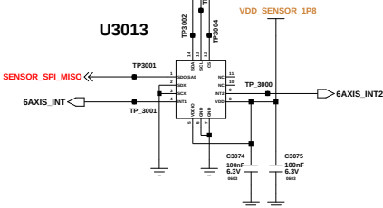
6 AXIS(ACC+GRYO) STM(3x2.5)
