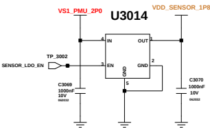
SENSOR LDO
